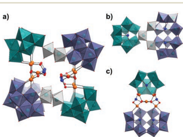
Fig. 1 Combined polyhedral/ball and stick representation of the structure of 1 showing; (a) front view of the intact cluster [H_{12}Pd_{10}Se_{10}W_{52}O_{206}]^{26-} , (b) top-down view of one \{Se_3W_{26}\} half-unit and, (c) side-on view of the (\{SeW_9\}\{Pd_5Se_2\}\{Se_2W_{14}\}) half-unit with the \{WO_6\} linkers removed for clarity. (Colour code: \{SeW_9\} units: teal polyhedra, \{Se_2W_{14}\} units: purple polyhedra, WO_6 linkers: grey polyhedra, Pd = orange, Se = blue, O = red. Cations and water molecules have been omitted for clarity.)
