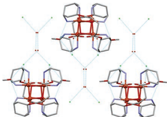
Figure 12. Packing of hydrogen-bonded subunits parallel to the crystallographic c axis (viewed from the a axis) in [\{Cu_2(OH)_2(GADACE)_2\}_2]Cl_4 \cdot 2MeOH \cdot 6H_2O , 6 . Color codes as in Figure 3.
