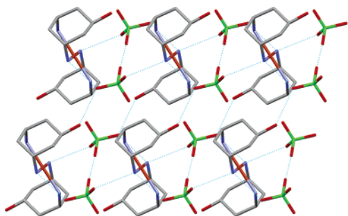
Figure 3. Hydrogen-bonded layer in anti -[Cu(DAHC) 2 ](ClO 4 ) 2 (1), viewed along the crystallographic c axis: C, gray; O, red; N, blue; Cl, green; Cu, copper; H, omitted. Hydrogen bonds are shown as bright blue dotted lines between the donor/acceptor positions.
