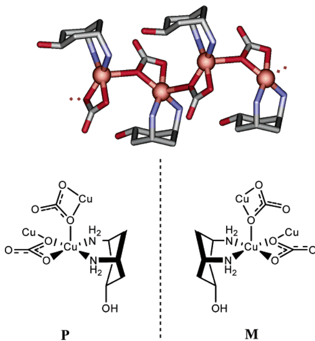
Figure 13. The [\{Cu(DAHC)(CO_3)\}_n] polymer, 7 : (top) assembly of [Cu(DAHC)(CO_3)] units into a chain and (bottom) the chiral copper(II) center in 7 .
