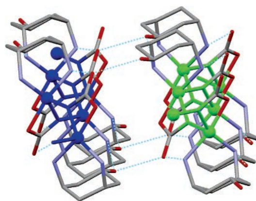
Figure 14. Association of the P- and M-enantiomers of [Cu(DAHC)(CO_3)]_n , 7 , to form a hydrogen-bonded layer. Cu and \mu -O are blue (P) or green (M); other color codes as in Figure 3.
