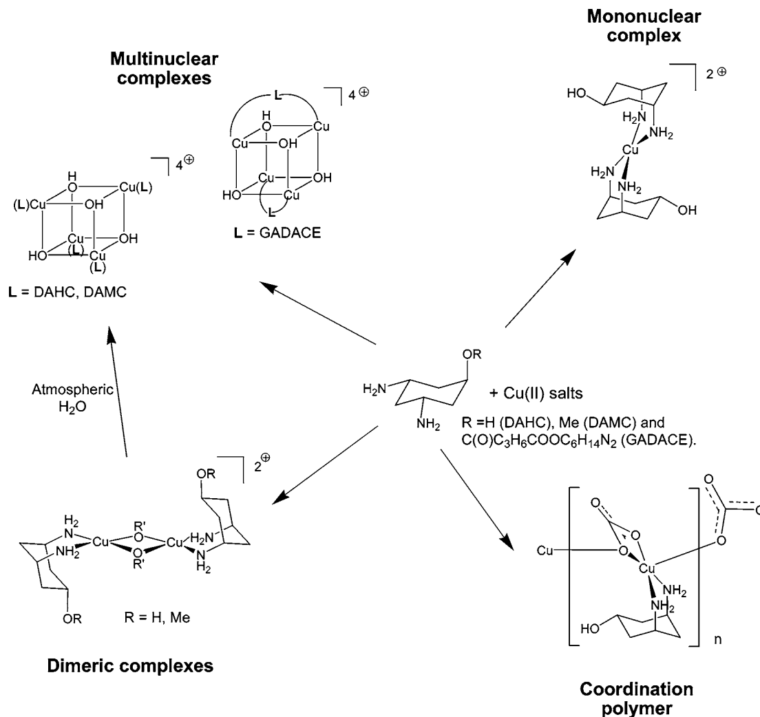
Figure 15. Summary of the coordination chemistry of the DAHC, DAMC, and GADACE ligands with \text{Cu}^{\text{II}} .
