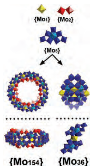
Figure 1. Scheme showing the assembly of the parent MB nanoring \{Mo_{154}\} (left), and the \{Mo_{36}\} unit (right) from transferrable building blocks. Color scheme: \{Mo_1\} , yellow; \{Mo_2\} , red; \{Mo_8\} , blue (central MoO_7 pentagonal bipyramid, light blue).
