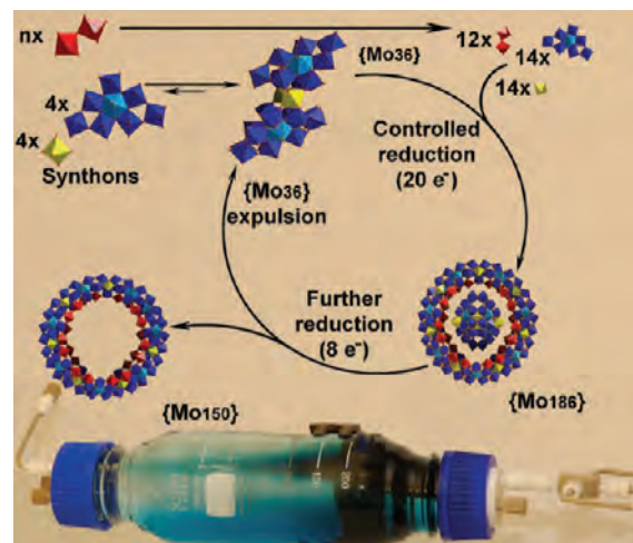
Figure 2. Scheme showing the assembly of a MB nanoring, complete with \{Mo_{36}\} template under continuous flow conditions. Color scheme: \{Mo_1\} , yellow; \{Mo_2\} , red; \{Mo_8\} , blue (central MoO_7 pentagonal bipyramid, light blue). Background shows the flow reactor setup used in our studies.
