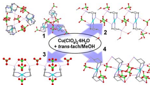
Fig. 2. Summary of compounds 1 – 4 . Colour scheme: chlorine atoms are in light green, oxygen atoms are in red, carbon atoms in grey and nitrogen atoms in blue. Inter -complex hydrogen-bonding interactions are shown as pink dashed lines (colour online).
