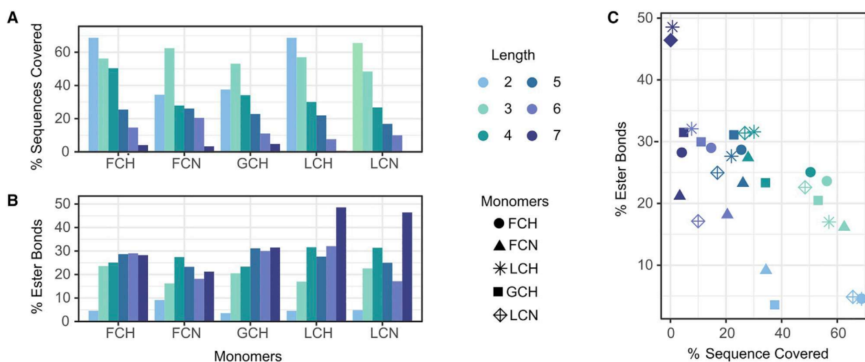
Figure 4. Sequence diversity
