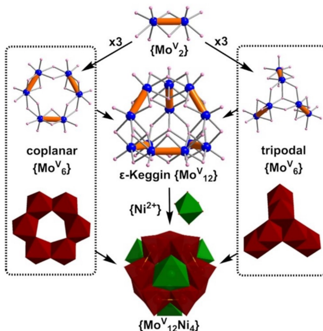
Figure 1. Schematic representation of the formation of the different building blocks that produce the ε-Keggin anion, [Mo 12 H 12 O 40 ] 8- , and its Ni-capped derivative structure, {Mo 12 Ni 4 }. Mo V : blue balls and brown polyhedra. Ni: dark green balls and polyhedra. O: pink balls.
