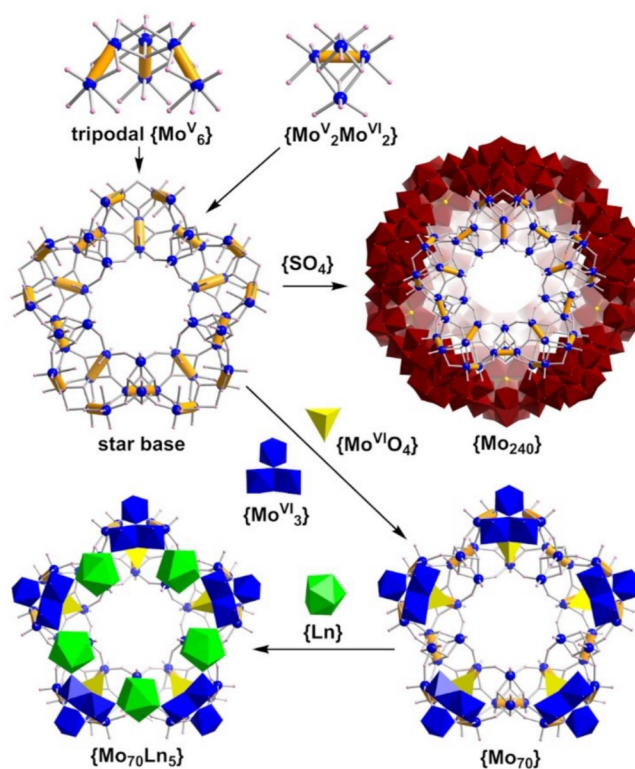
Figure 4. Schematic representation of the formation of the star compounds, 4 , 5 and 6 . Star base is the common part for forming \{\text{Mo}_{70}\} and \{\text{Mo}_{240}\} . Colour scheme is the same as that in Figure 2.
