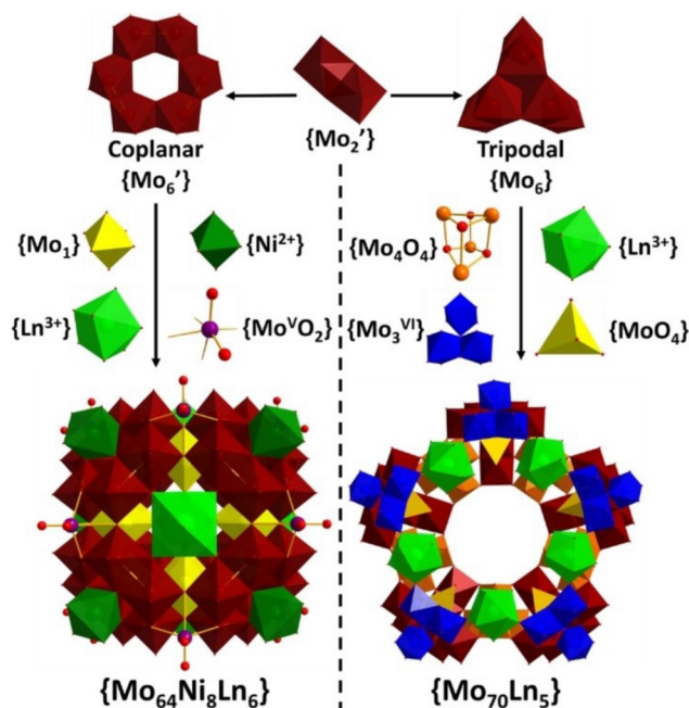
Figure 2. Schematic representation of the formation of compounds 1 to 6 . Left side: compounds 1 – 3 . Right side: compounds 4 – 6 . Mo V : maroon balls and polyhedra. {Mo VI }: yellow or blue polyhedra. {Mo V O 2 }: purple ball. Ni: dark green polyhedra. Ln: light green balls and polyhedra. O: red balls.
