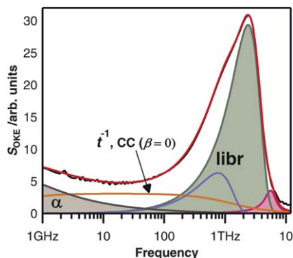
Fig. 4 Fit (red) of the OKE spectrum (black) for PAN at 200 K. CC is the Cole-Cole function with \beta = 0 as described in the text.
