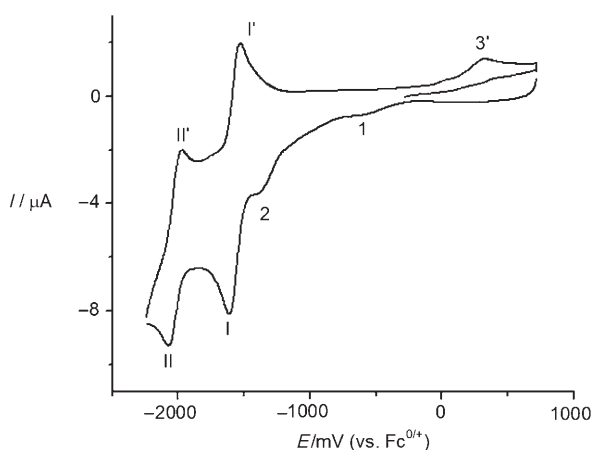
Figure 3. Cyclic voltammogram of 1 mM (TBA) 6 [H 3 W 18 O 56 (IO 6 )] 2' in CH 3 CN (0.1 M THAClO 4 ) on a glassy carbon electrode at a scan rate of 100 mVs -1 . The two redox potentials associated with I/I' and II/II' are -1.57 and -2.02 V, respectively. Two small processes (1 and 2) are seen when the potential was scanned from positive to negative, but disappear after further scans. These processes are associated with protonated species derived from the POM itself or from enhanced levels of protonation associated with the presence of adventitious water in the solvent. A small oxidation process (3) was observed when switching potential after reduction process I (origin unknown).
