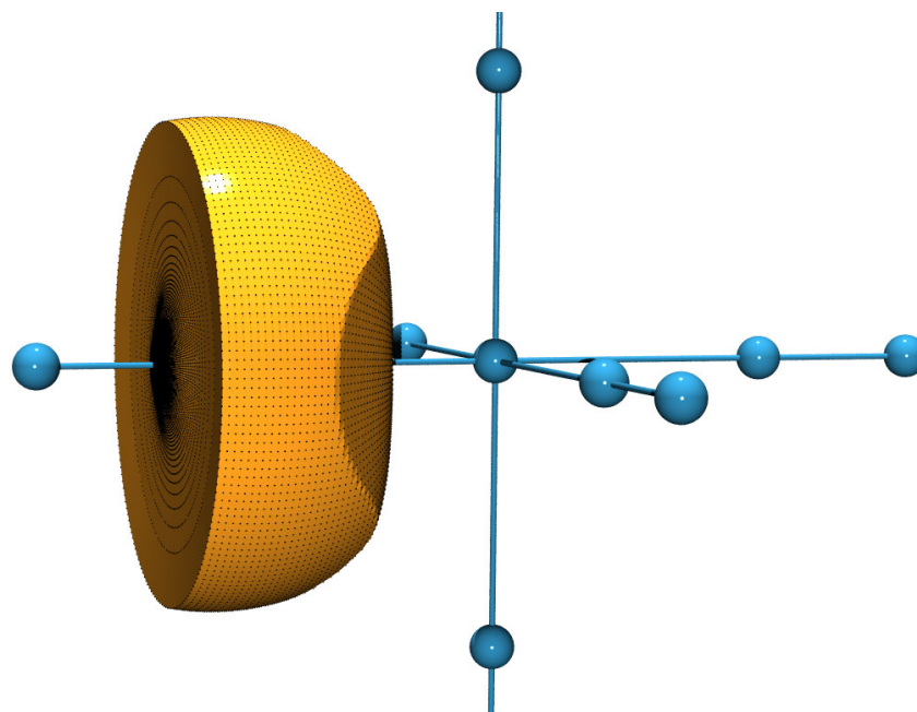
Figure 10-3. Atomic basin of C atom in \text{Cr}(\text{CO})_6 using the utilities program rays2pov.
